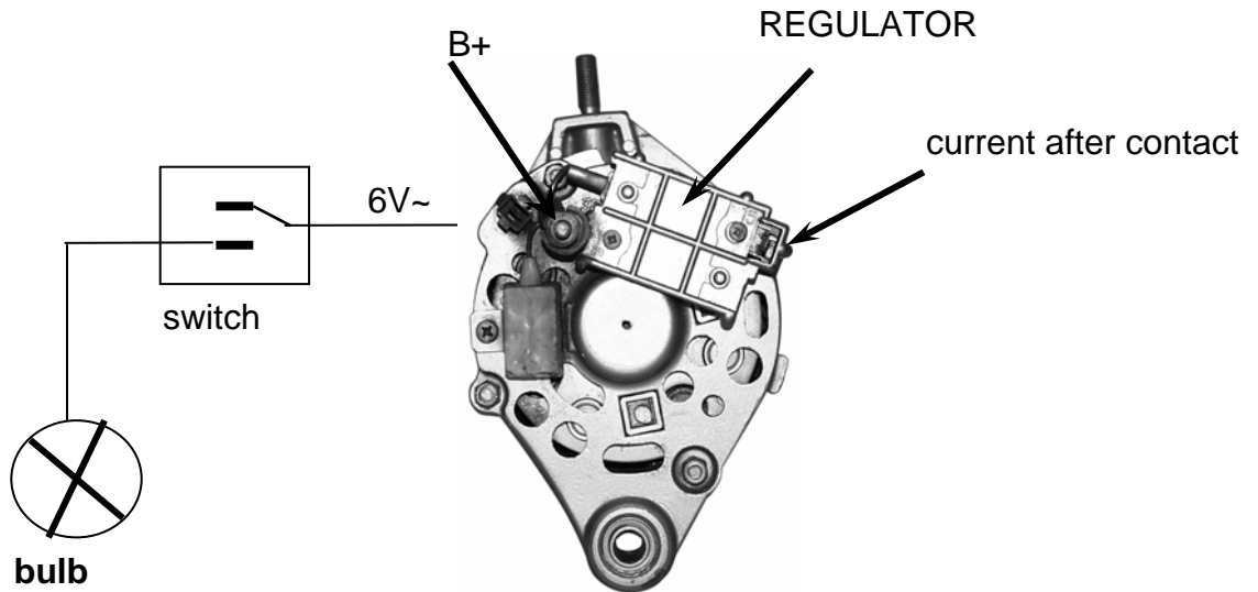
Alternator without field diodes
